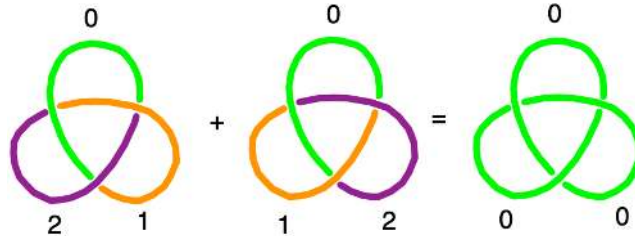
Figure 9. Adding 3-colorings
